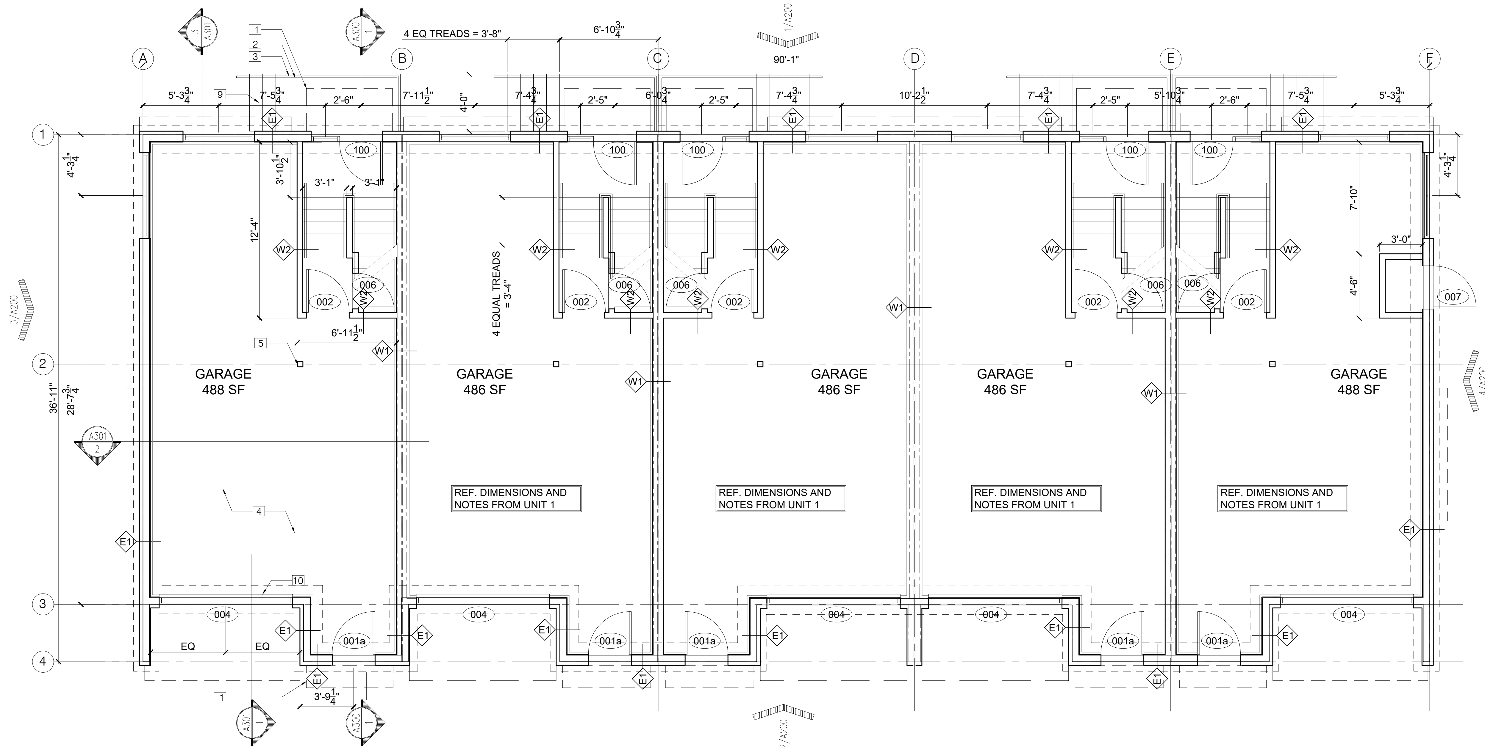
1 BUILDING "A" FIRST FLOOR 0 4'-0" SCALE: 1/4" = 1'-0"
