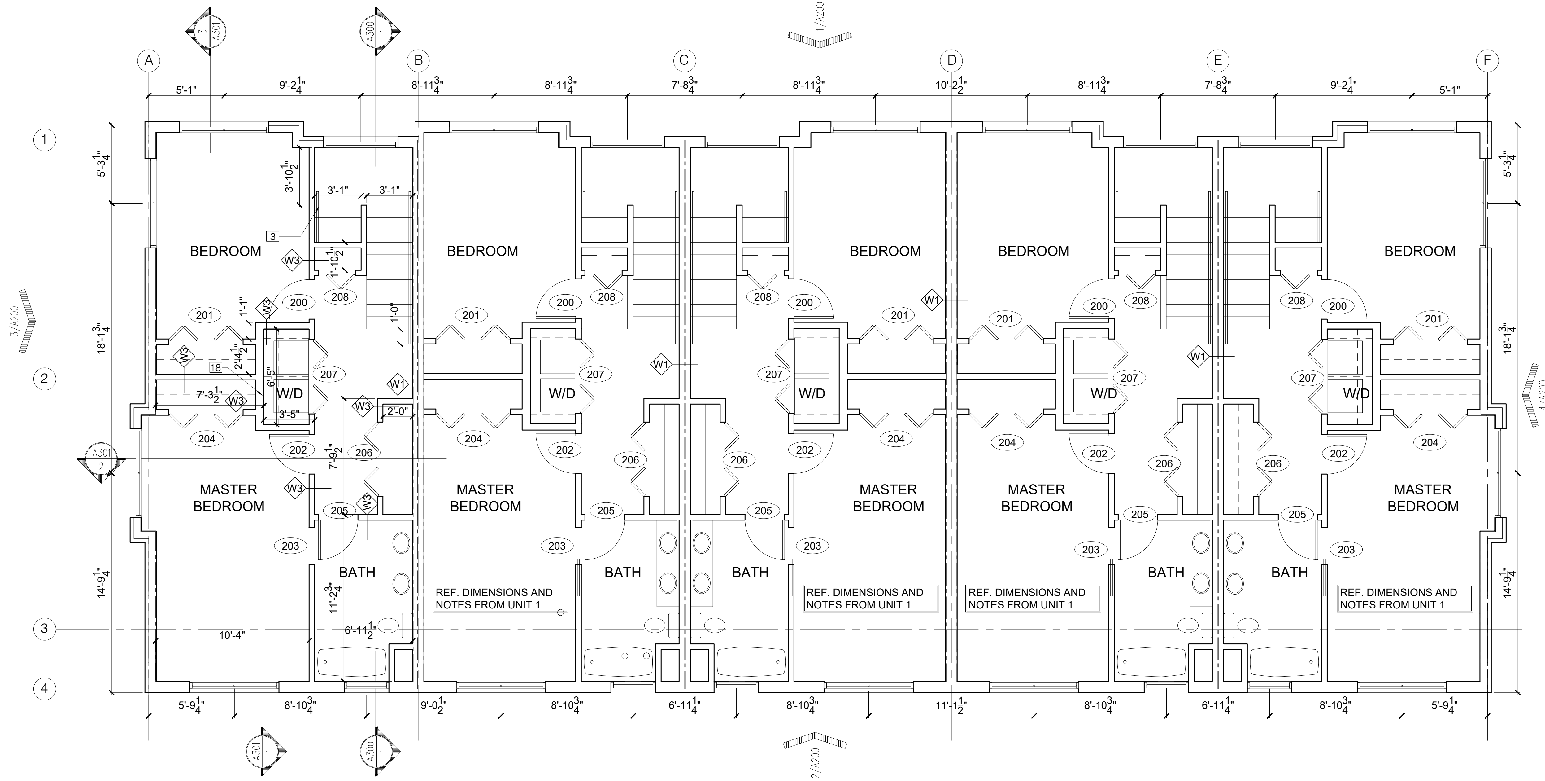
1 BUILDING "A" THIRD FLOOR 0 4'-0" SCALE: 1/4" = 1'-0"
